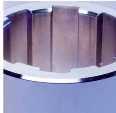
Spline profile
