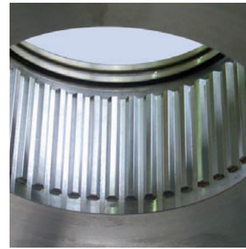
Involute profile
