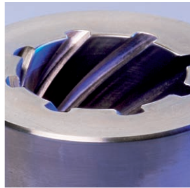
Helical keyway
