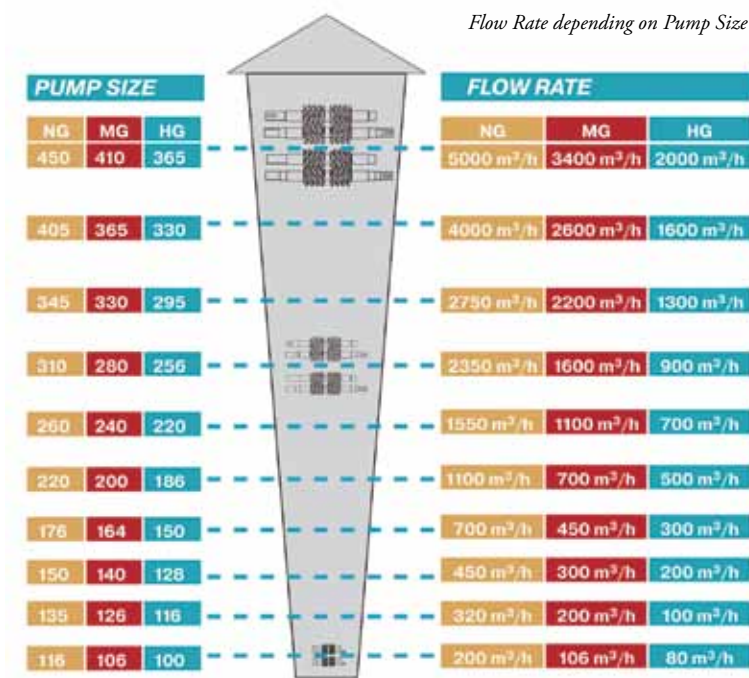
Flow Rate depending on Pump Size
