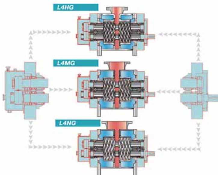
Modular System for Leistriz L4 Series Twin Screw Pumps
